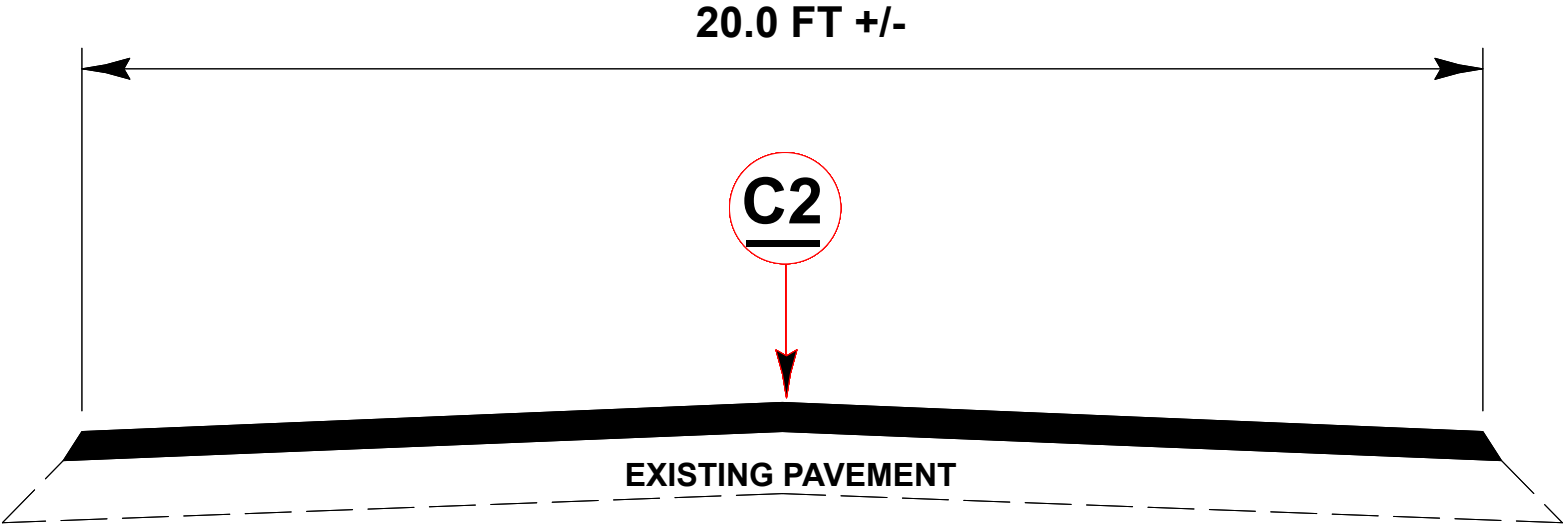
TYPICAL SECTION # 2 MAP(S) # 4 & 6 - 8
