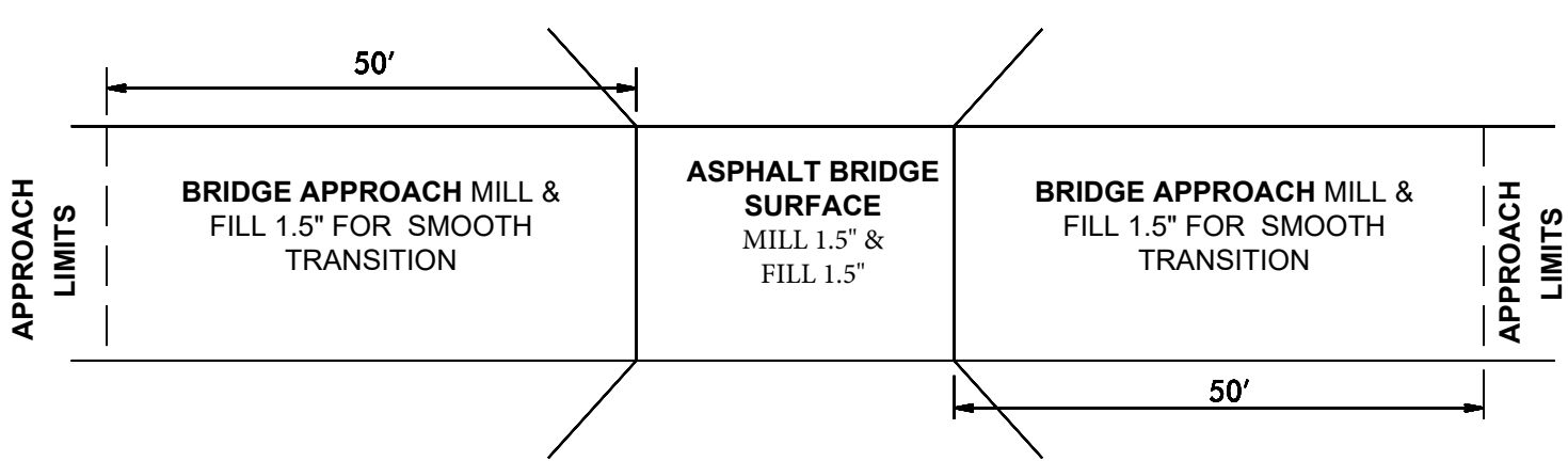
DETAIL FOR MAP # 3 & 4 / STRUCTURE # 0059 & 0037
