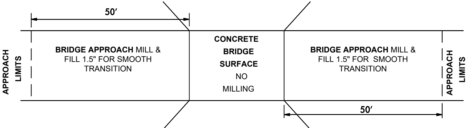
DETAIL FOR MAP # 1 & 3 / STRUCTURE # # 0012 & # 0243
